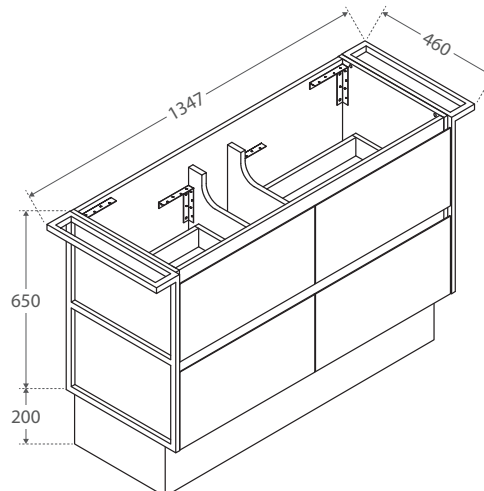
1200 with twin towel rail frames
