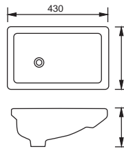
Edge Mini VCB540C Underbench 430x255 w/overflow (extra charge)
