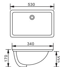
Elegant VCB540E Underbench 530x340 w/overflow (extra charge)
